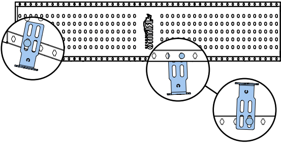
LP03
