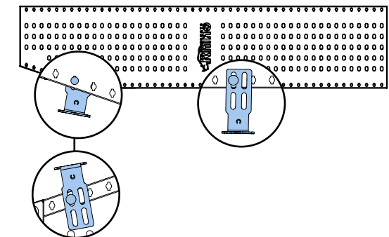
LP01
