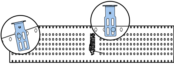
LP05
