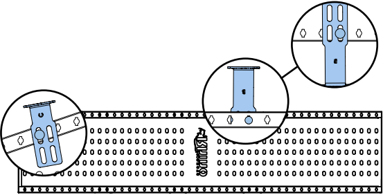
LP02
