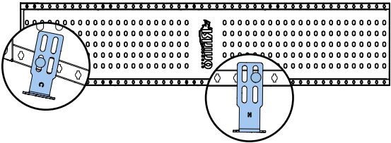
LP04
